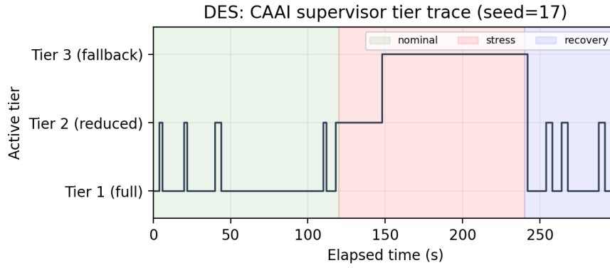
Fig. 9: Discrete-event simulation: CAAI supervisor-selected tier vs. elapsed time for the representative run (seed = 17). Shaded regions mark nominal (0–120 s), stress (120–240 s), and recovery (240–300 s) phases.
